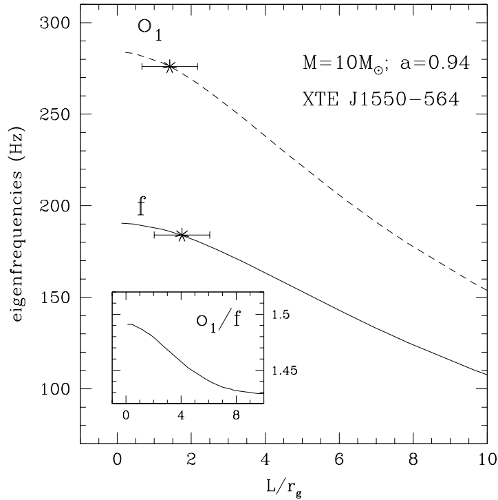
FIGURE 1. p -mode frequencies for a non-Keplerian disc. The horizontal axis shows the normalized radial dimensions of the torus L/r_g when the black hole has a mass M = 10 M_\odot . The fundamental frequencies f are indicated with a solid line, while the first overtones o_1 with a dashed line. The filled dot indicates the epicyclic frequency at r_{\max} , while the two asterisks show the values of the HFQPOs observed in XTE J1550-546. The error bars show the uncertainty in the determination of M .
